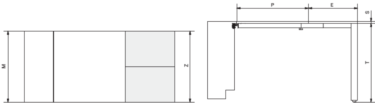
Dinamico+ PROFILO GOLA + STAFFE + MECCANISMO ALLUNGABILE + GAMBA GOLA PROFILE + BRACKETS + EXTENDABLE MECHANISM + LEG
