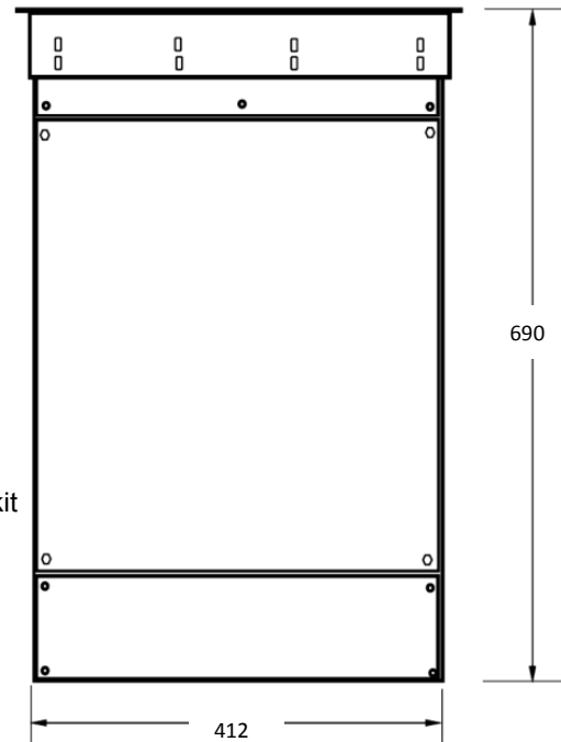
OPTION B Flush with work surface. Approx. 3mm rebate. Standard Collar
