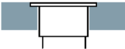
OPTION B Flush with work surface. Approx. 3mm rebate. Standard Collar
